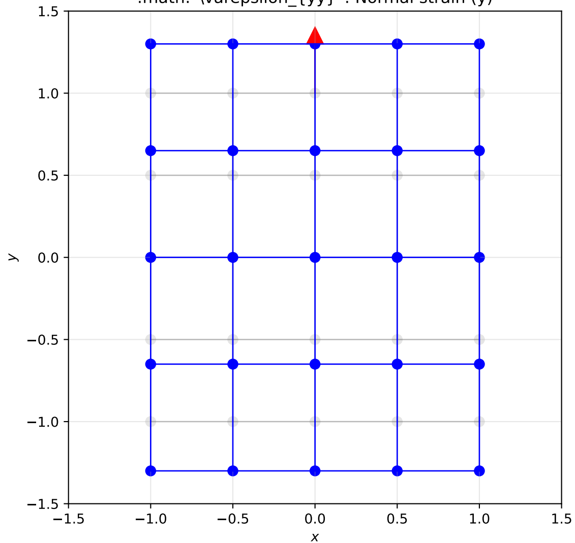
\epsilon_{yy} : Normal strain (y)
