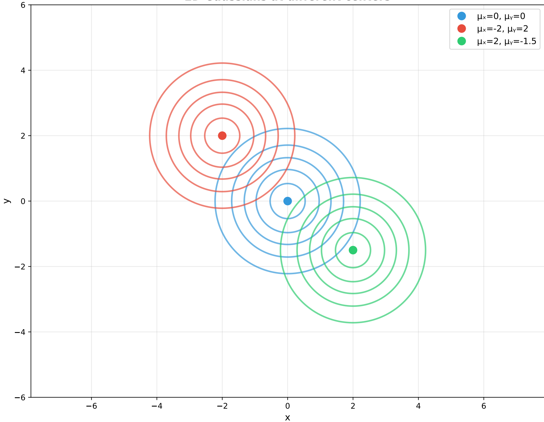
2D Gaussians at different centers
