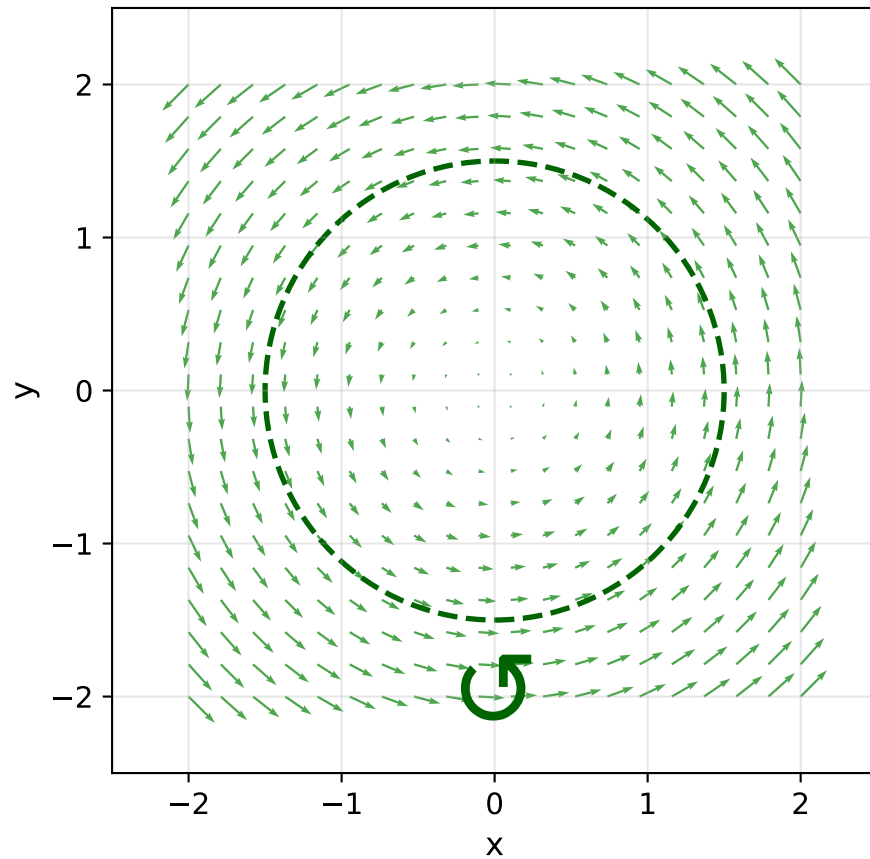
Zero Divergence \nabla \cdot \mathbf{F} = 0.0 (Incompressible)
