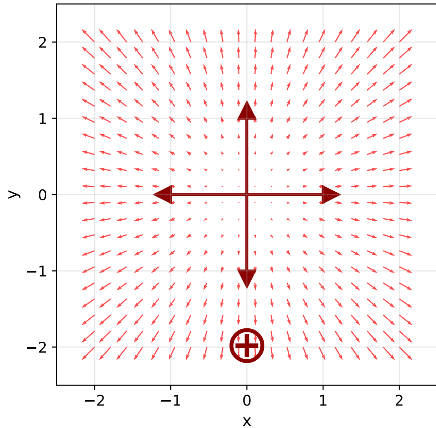
Positive Divergence \nabla \cdot \mathbf{F} = 2.0 (Source)
