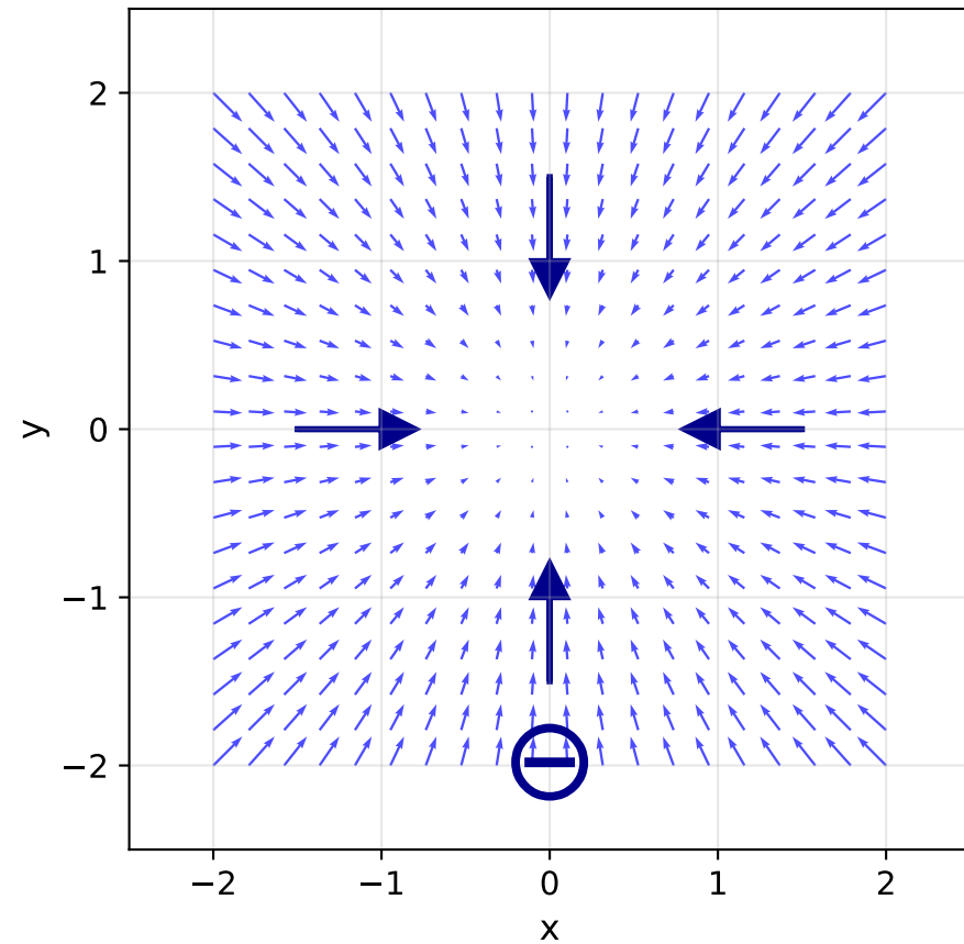
Negative Divergence \nabla \cdot \mathbf{F} = -2.0 (Sink)
