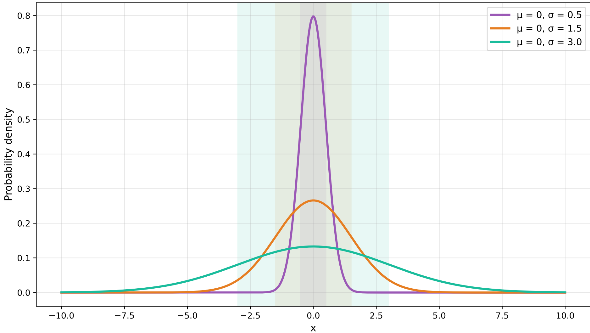
Effect of changing standard deviation \sigma
