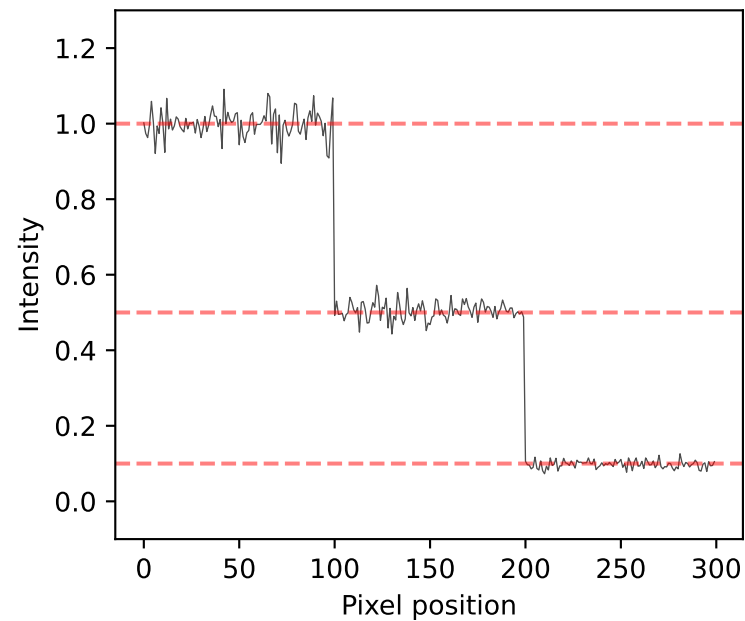
SNR: 31.6×
