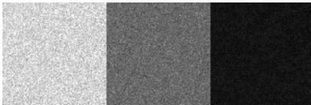
\lambda = 100 (dose)
