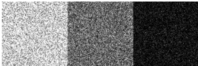
\lambda = 10 (dose)
