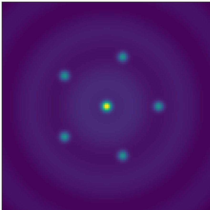
Inelastic Scattering
