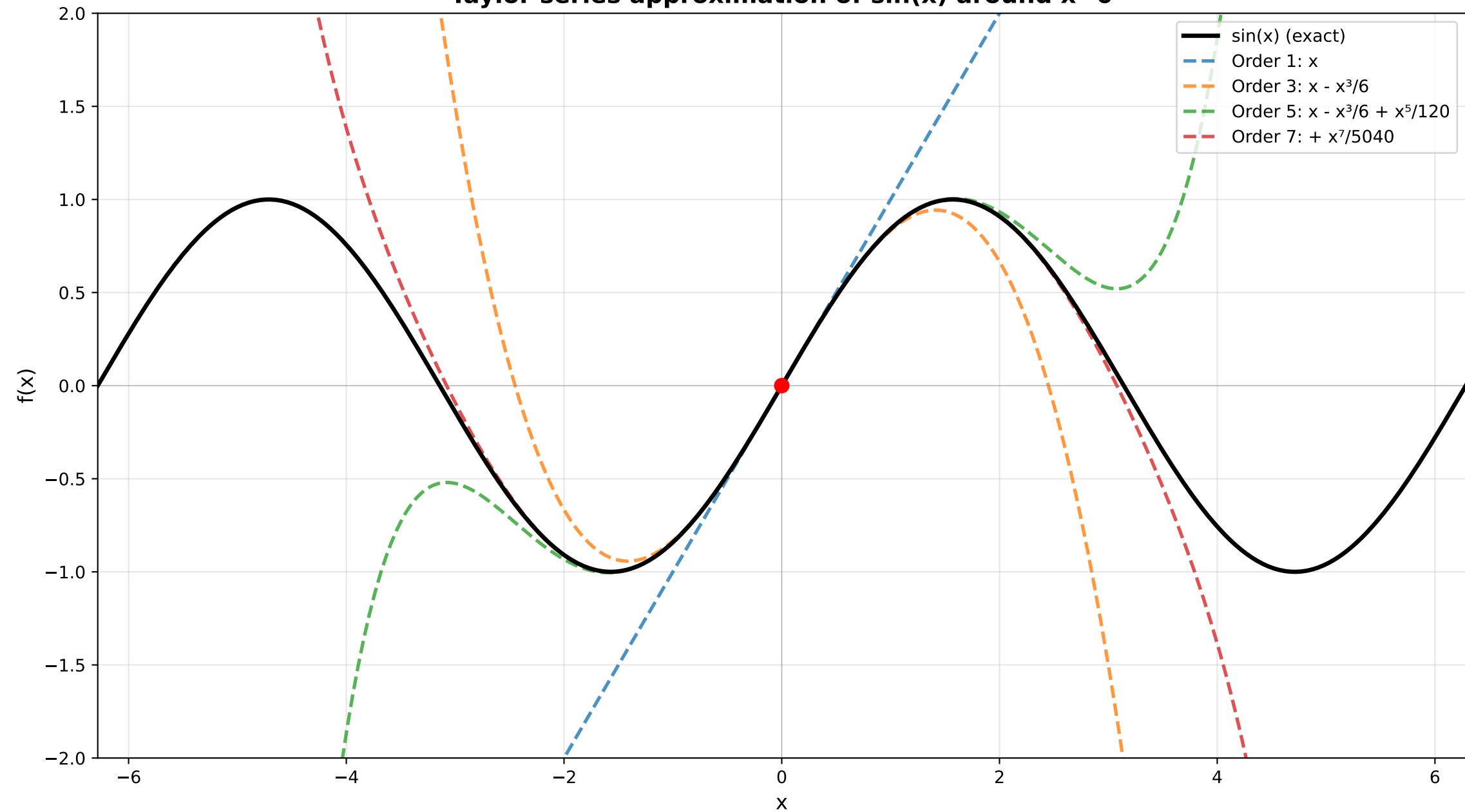
Taylor series approximation of \sin(x) around x=0
